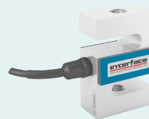
SSM or SSM2 Sealed S-Type Load Cell 50 lbf to 10K lbf 200 N to 50 kN
